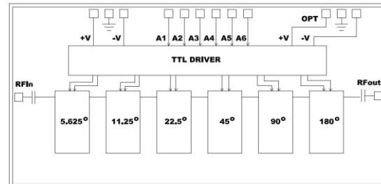
Functional diagram
